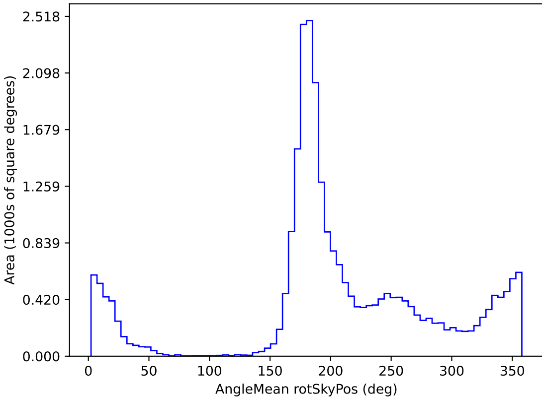
smc_lmc_v3.3_10yrs All sky z band: AngleMean rotSkyPos
