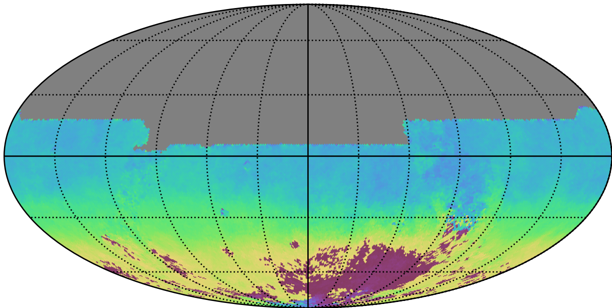
smc_lmc_v3.3_10yrs All sky y band: AngleMean rotSkyPos
