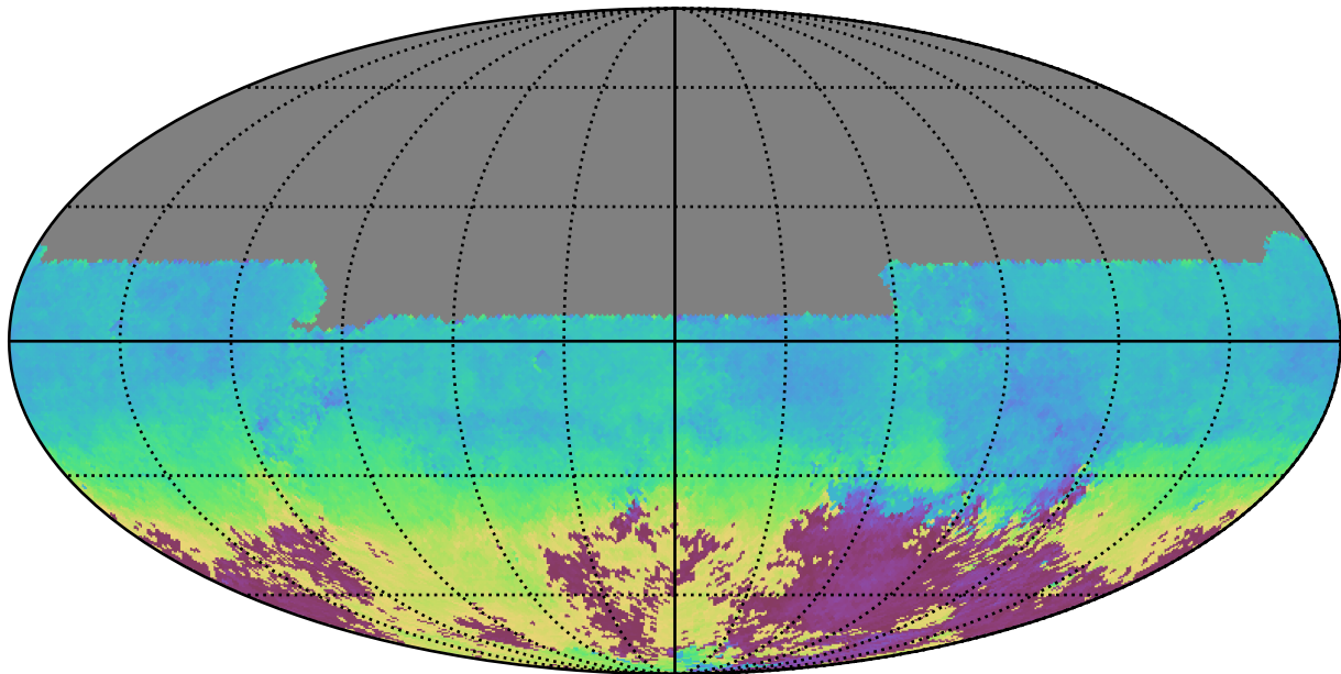
smc_lmc_v3.3_10yrs All sky u band: AngleMean rotSkyPos
