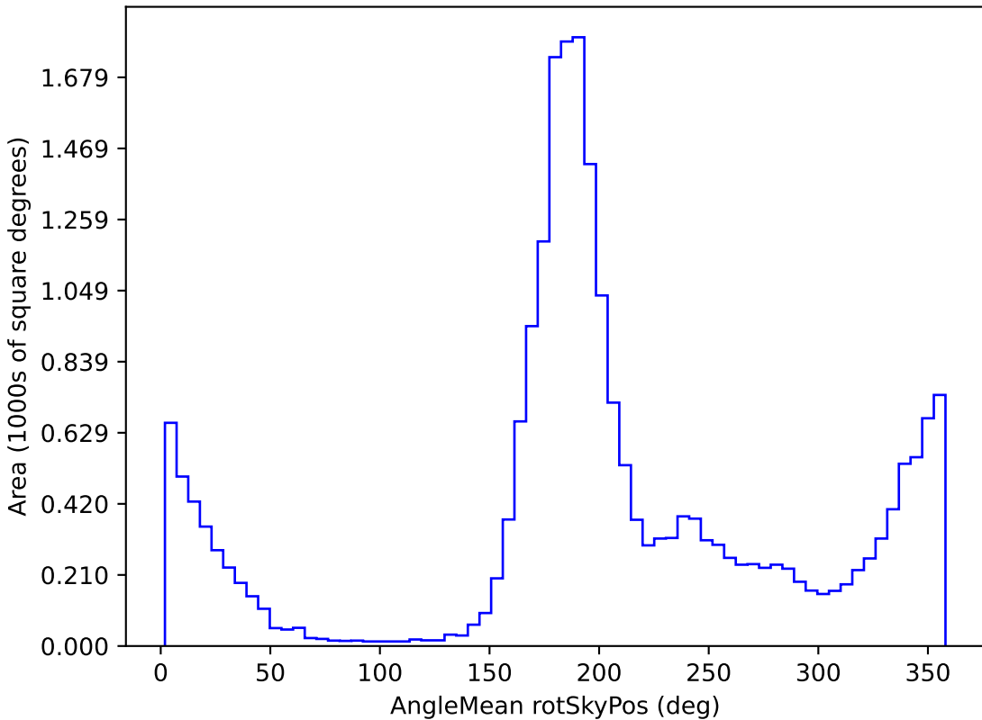
smc_lmc_v3.3_10yrs All sky u band: AngleMean rotSkyPos
