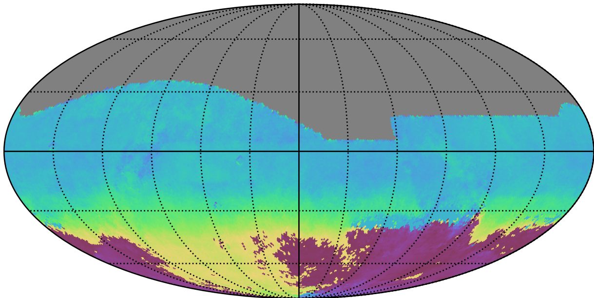
smc_lmc_v3.3_10yrs All sky r band: AngleMean rotSkyPos
