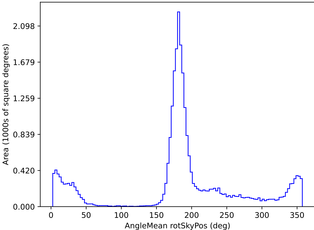
smc_lmc_v3.3_10yrs All sky r band: AngleMean rotSkyPos
