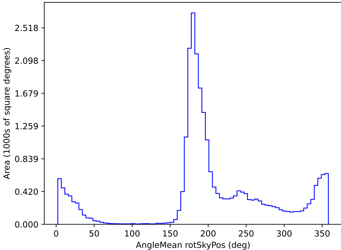
smc_lmc_v3.3_10yrs All sky i band: AngleMean rotSkyPos
