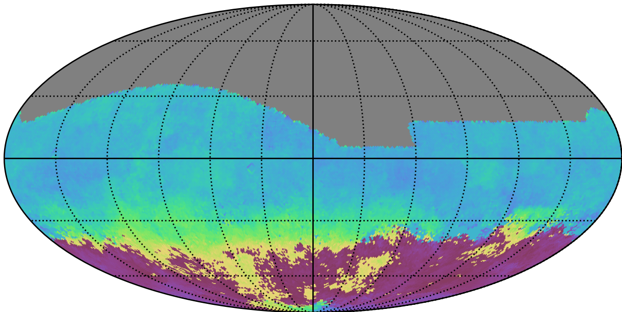
smc_lmc_v3.3_10yrs All sky g band: AngleMean rotSkyPos
