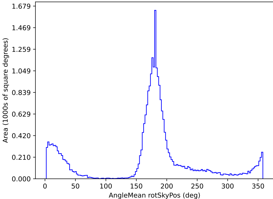
smc_lmc_v3.3_10yrs All sky g band: AngleMean rotSkyPos
