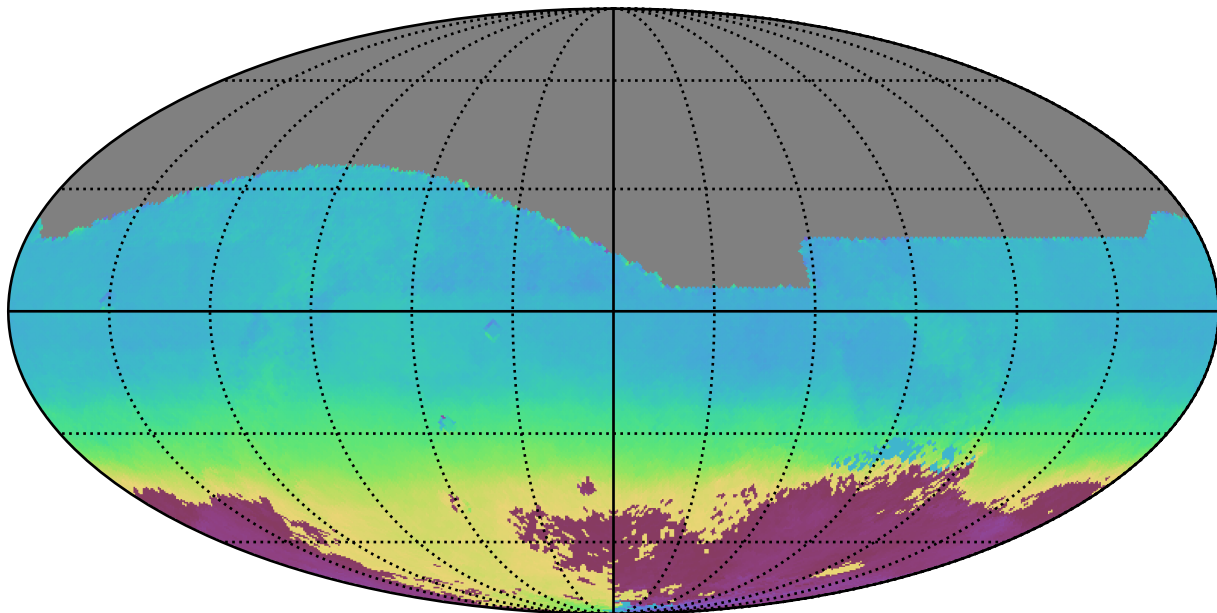
smc_lmc_v3.3_10yrs All sky all bands: AngleMean rotSkyPos
