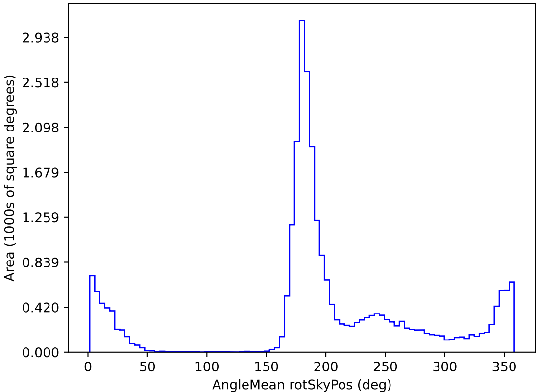
smc_lmc_v3.3_10yrs All sky all bands: AngleMean rotSkyPos
