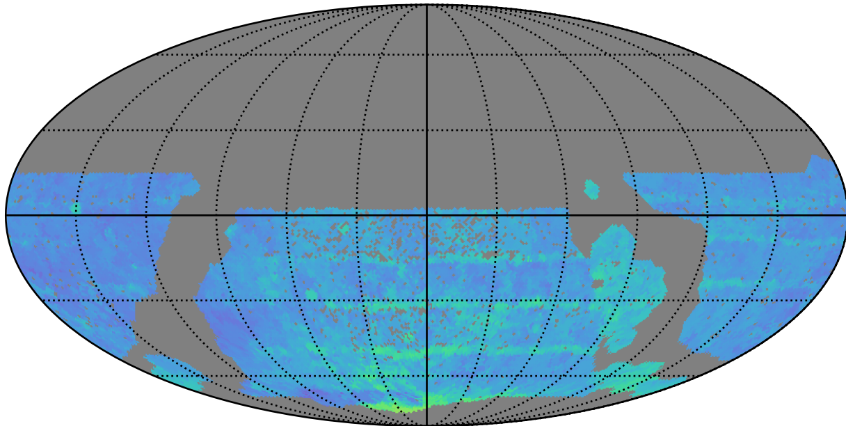
smc_lmc_v3.3_10yrs WFD z band: 80thPercentile Season Length
