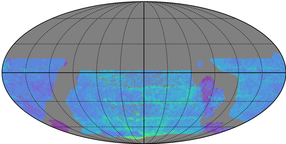
smc_lmc_v3.3_10yrs WFD y band: 80thPercentile Season Length
