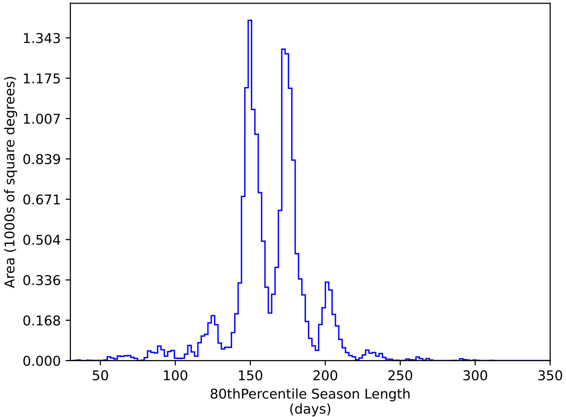
smc_lmc_v3.3_10yrs WFD y band: 80thPercentile Season Length
