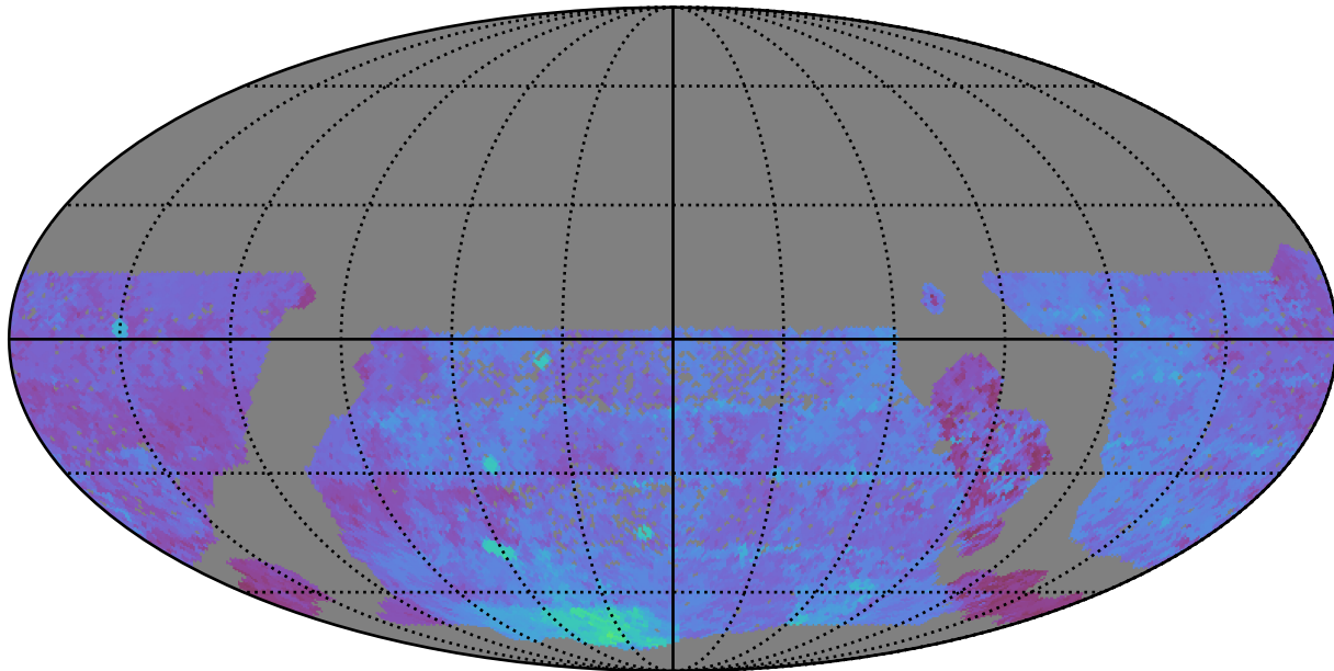
smc_lmc_v3.3_10yrs WFD u band: 80thPercentile Season Length
