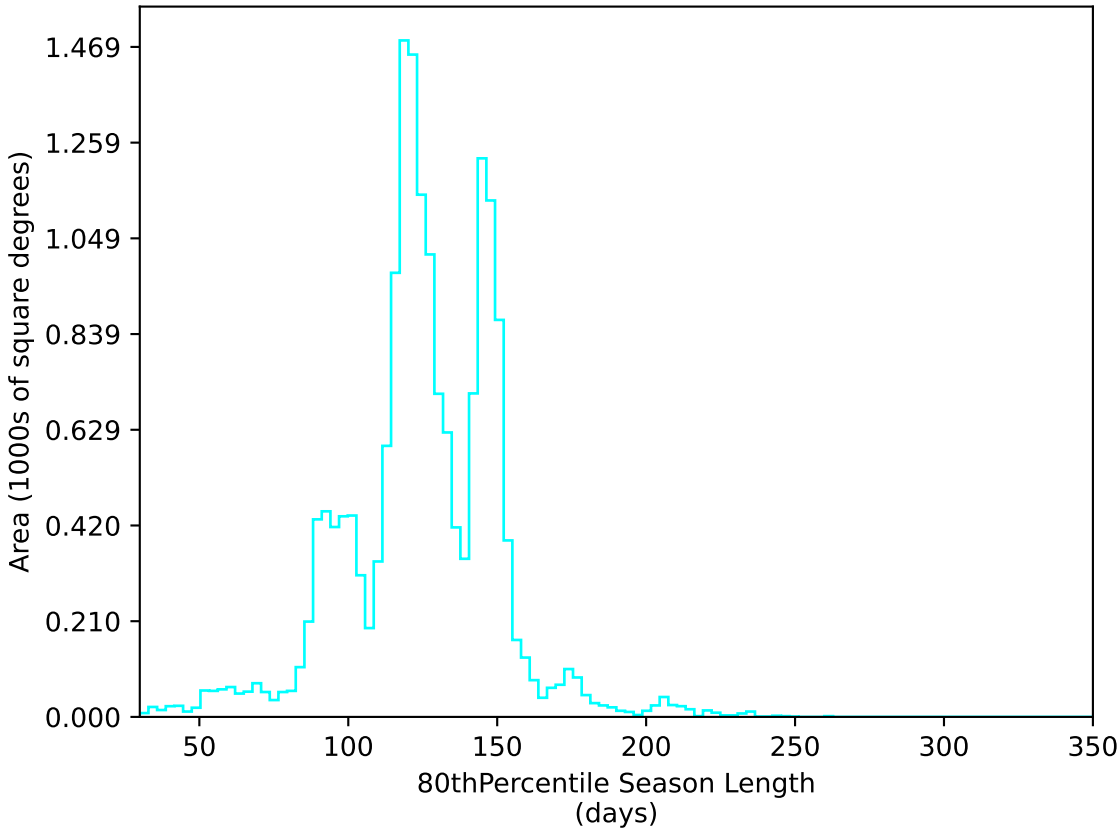
smc_lmc_v3.3_10yrs WFD u band: 80thPercentile Season Length
