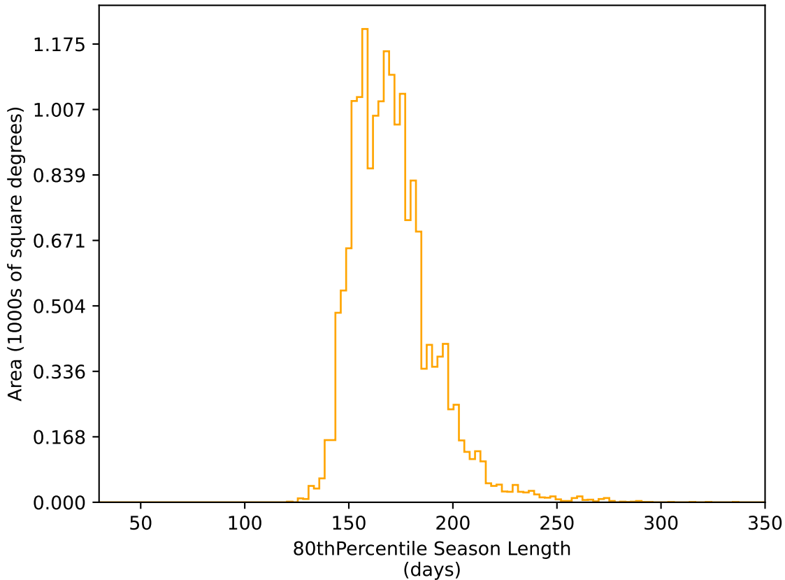
smc_lmc_v3.3_10yrs WFD r band: 80thPercentile Season Length
