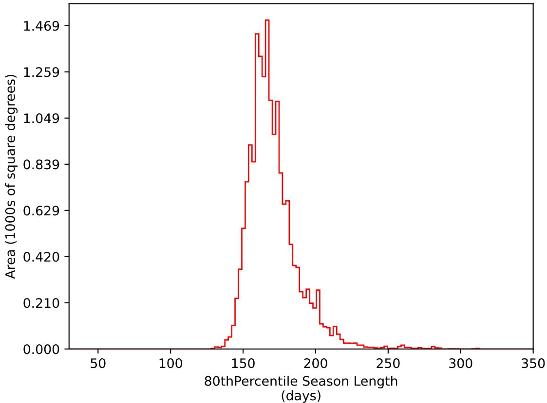
smc_lmc_v3.3_10yrs WFD i band: 80thPercentile Season Length
