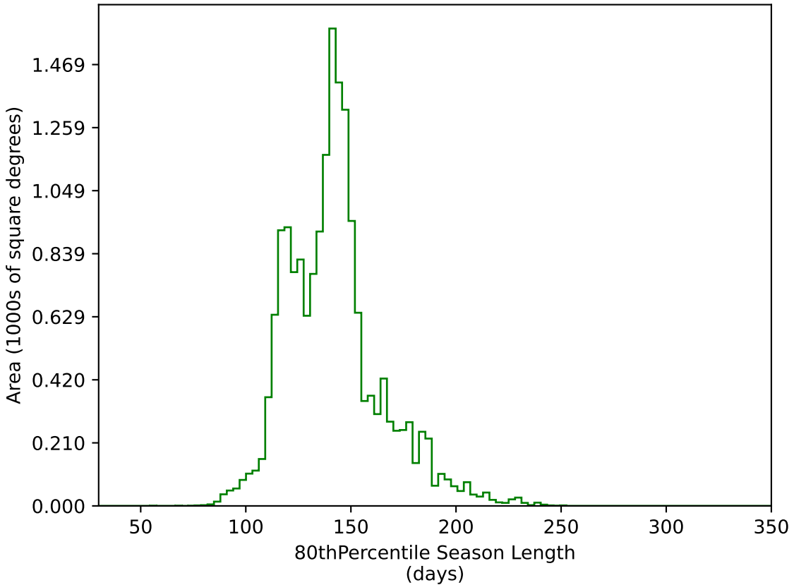
smc_lmc_v3.3_10yrs WFD g band: 80thPercentile Season Length
