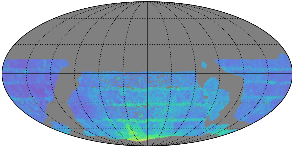
smc_lmc_v3.3_10yrs WFD all bands: 80thPercentile Season Length
