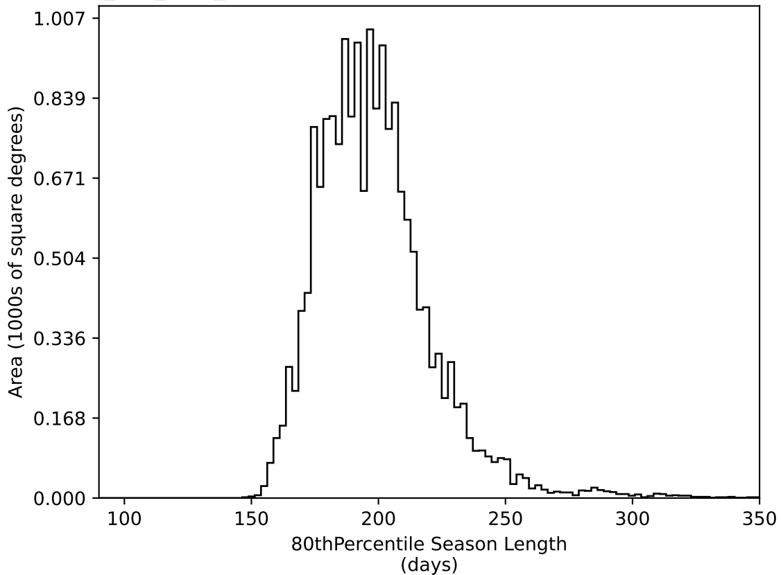
smc_lmc_v3.3_10yrs WFD all bands: 80thPercentile Season Length
