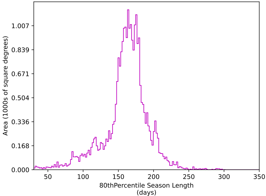
smc_lmc_v3.3_10yrs All sky z band: 80thPercentile Season Length
