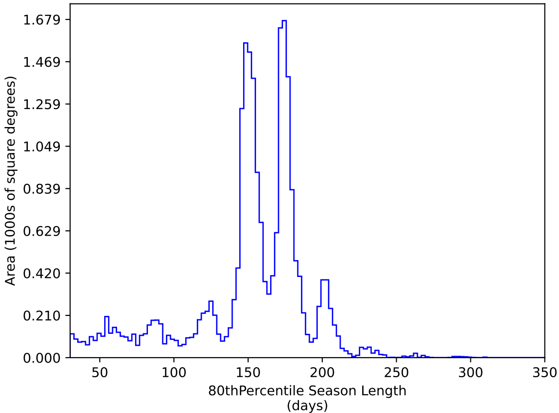
smc_lmc_v3.3_10yrs All sky y band: 80thPercentile Season Length
