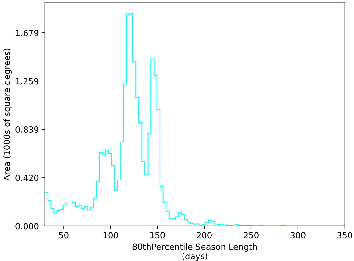
smc_lmc_v3.3_10yrs All sky u band: 80thPercentile Season Length
