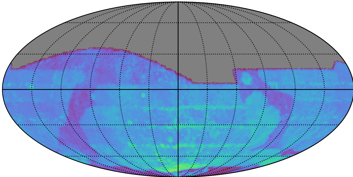
smc_lmc_v3.3_10yrs All sky r band: 80thPercentile Season Length
