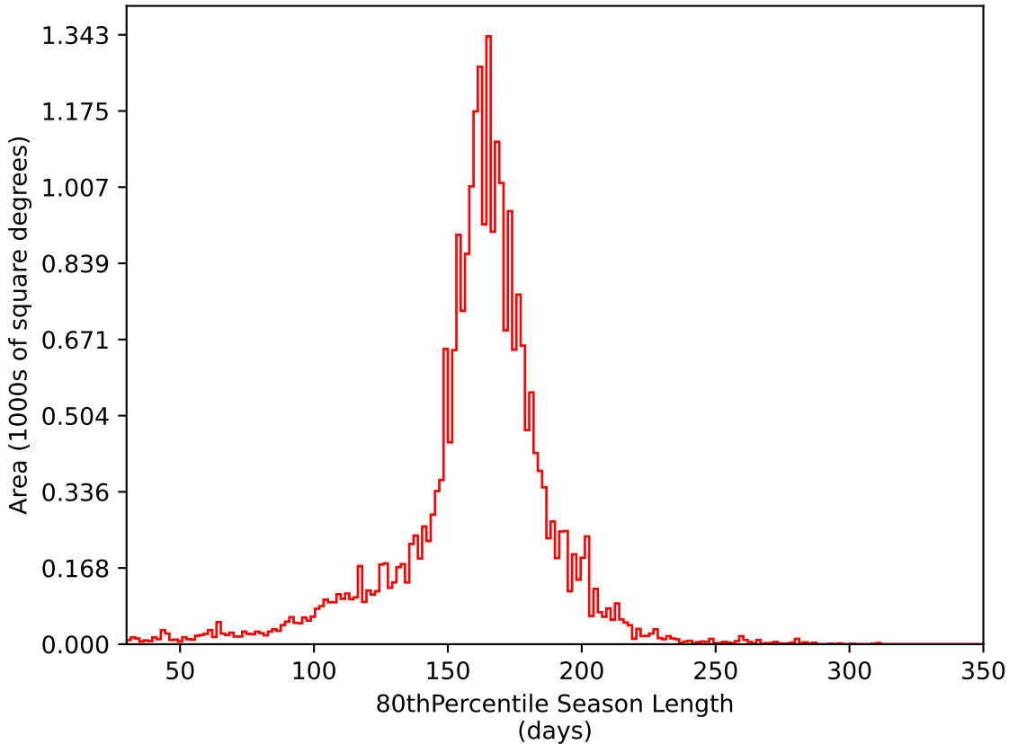
smc_lmc_v3.3_10yrs All sky i band: 80thPercentile Season Length
