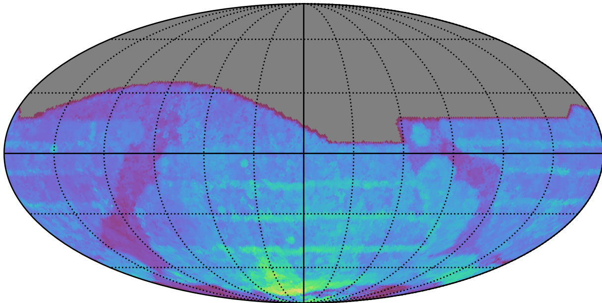
smc_lmc_v3.3_10yrs All sky all bands: 80thPercentile Season Length
