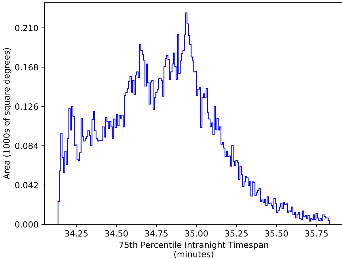
smc_Imc_v3.3_10yrs WFD zy bands: 75th Percentile Intranight Timespan
