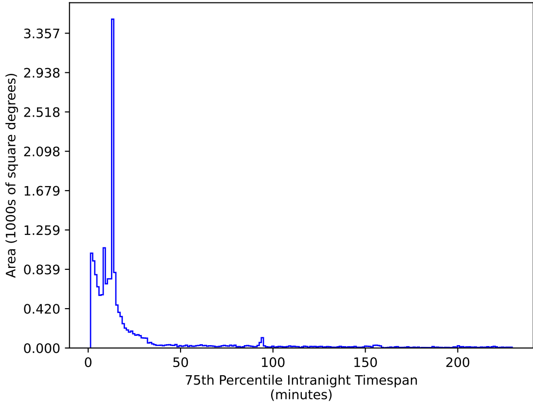
smc_lmc_v3.3_10yrs WFD z band: 75th Percentile Intranight Timespan
