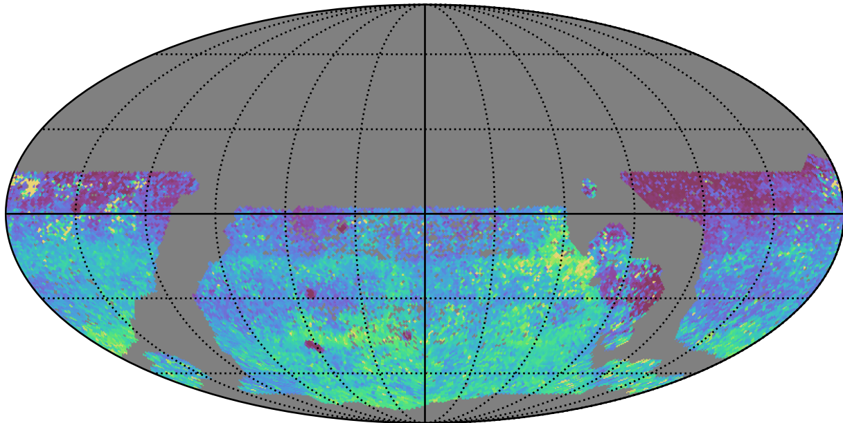
smc_lmc_v3.3_10yrs WFD y band: 75th Percentile Intranight Timespan
