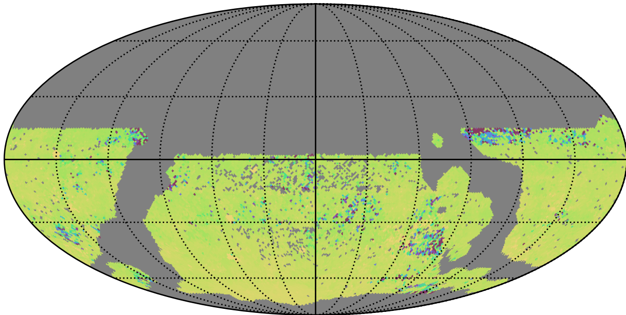
smc_lmc_v3.3_10yrs WFD ug bands: 75th Percentile Intranight Timespan
