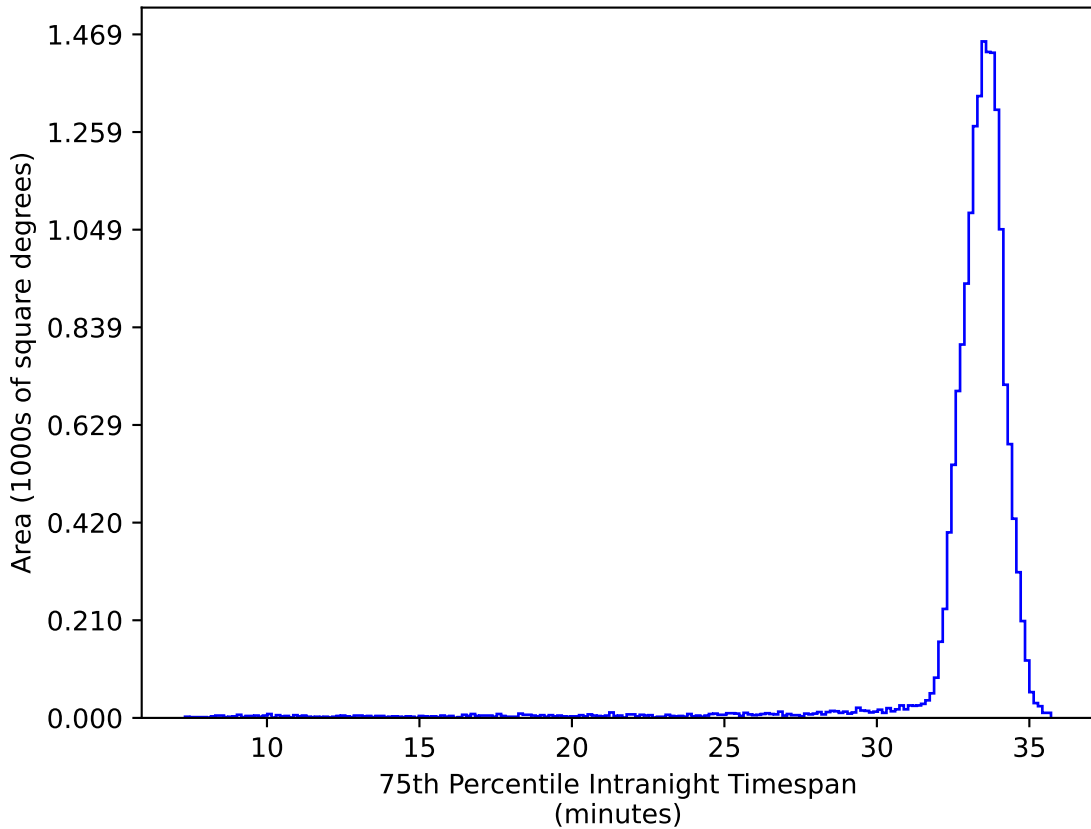
smc_Imc_v3.3_10yrs WFD ug bands: 75th Percentile Intranight Timespan
