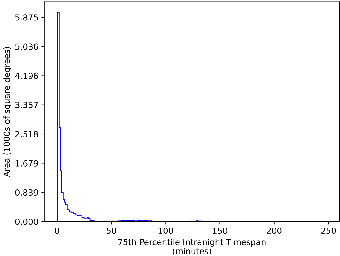
smc_lmc_v3.3_10yrs WFD u band: 75th Percentile Intranight Timespan
