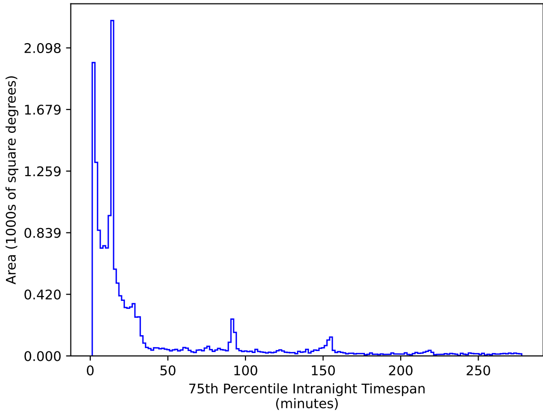
smc_lmc_v3.3_10yrs WFD r band: 75th Percentile Intranight Timespan
