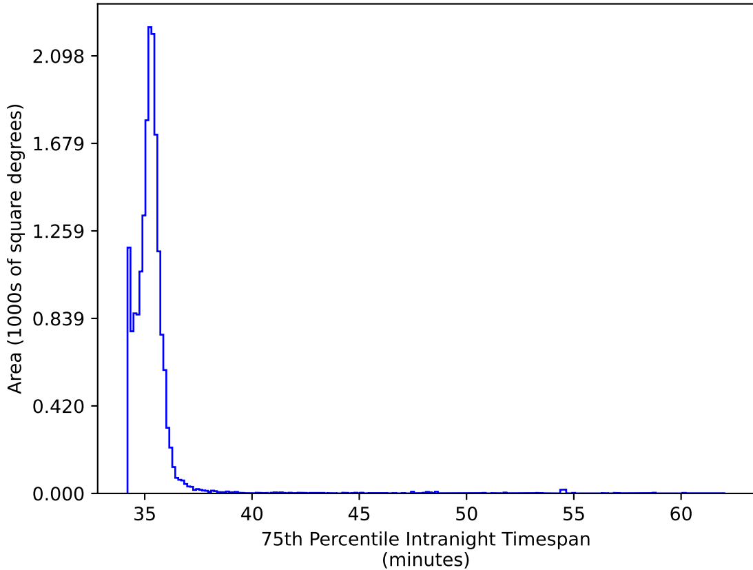
smc_lmc_v3.3_10yrs WFD iz bands: 75th Percentile Intranight Timespan
