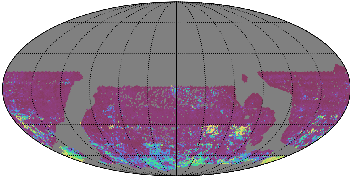
smc_lmc_v3.3_10yrs WFD i band: 75th Percentile Intranight Timespan
