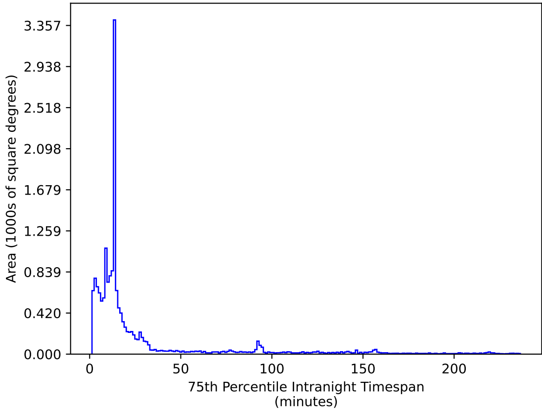
smc_lmc_v3.3_10yrs WFD i band: 75th Percentile Intranight Timespan
