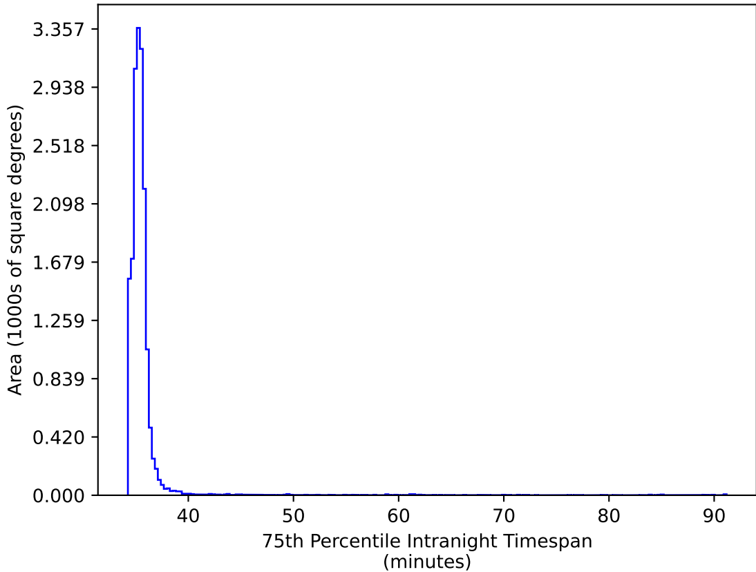
smc_Imc_v3.3_10yrs WFD gr bands: 75th Percentile Intranight Timespan
