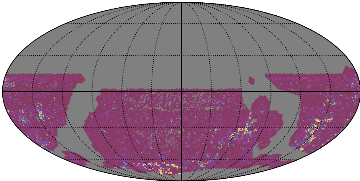
smc_lmc_v3.3_10yrs WFD g band: 75th Percentile Intranight Timespan
