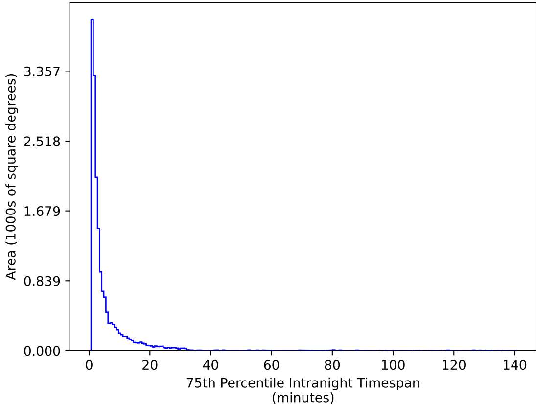
smc_lmc_v3.3_10yrs WFD g band: 75th Percentile Intranight Timespan
