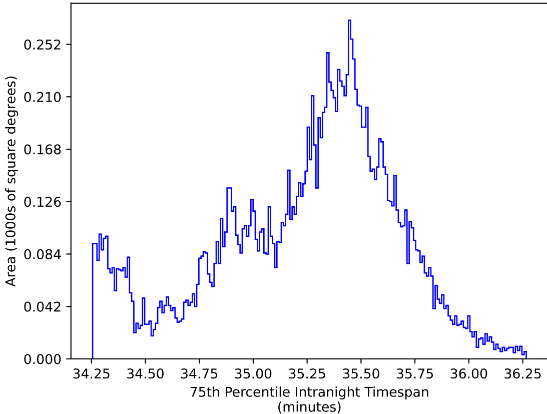
smc_Imc_v3.3_10yrs WFD all bands: 75th Percentile Intranight Timespan
