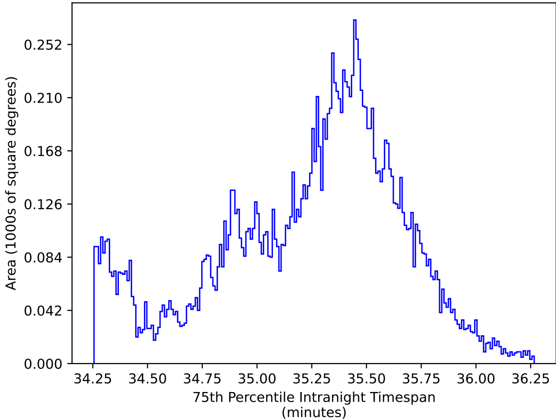
smc_lmc_v3.3_10yrs WFD: 75th Percentile Intranight Timespan
