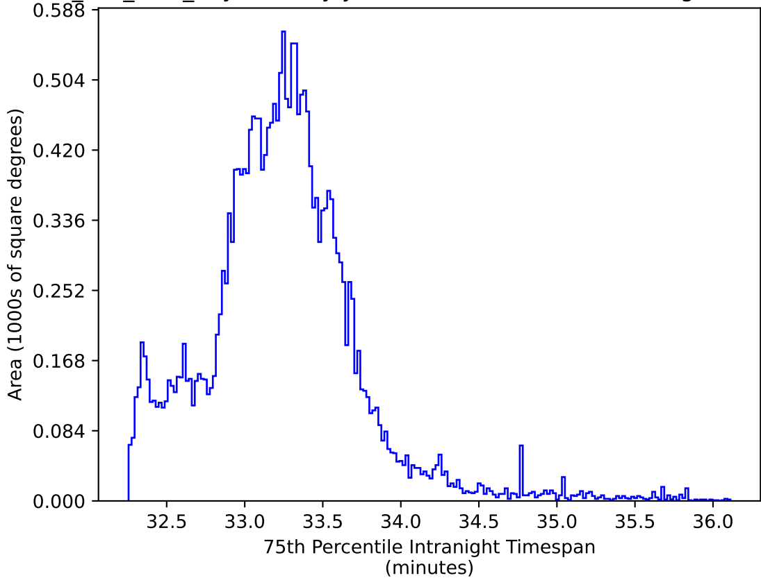
smc_lmc_v3.3_10yrs All sky y band: 75th Percentile Intranight Timespan
