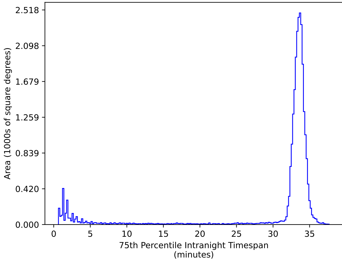
smc_lmc_v3.3_10yrs All sky ug bands: 75th Percentile Intranight Timespan
