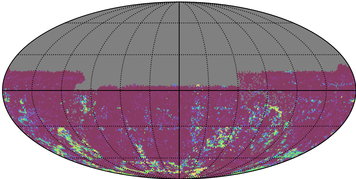
smc_Imc_v3.3_10yrs All sky u band: 75th Percentile Intranight Timespan
