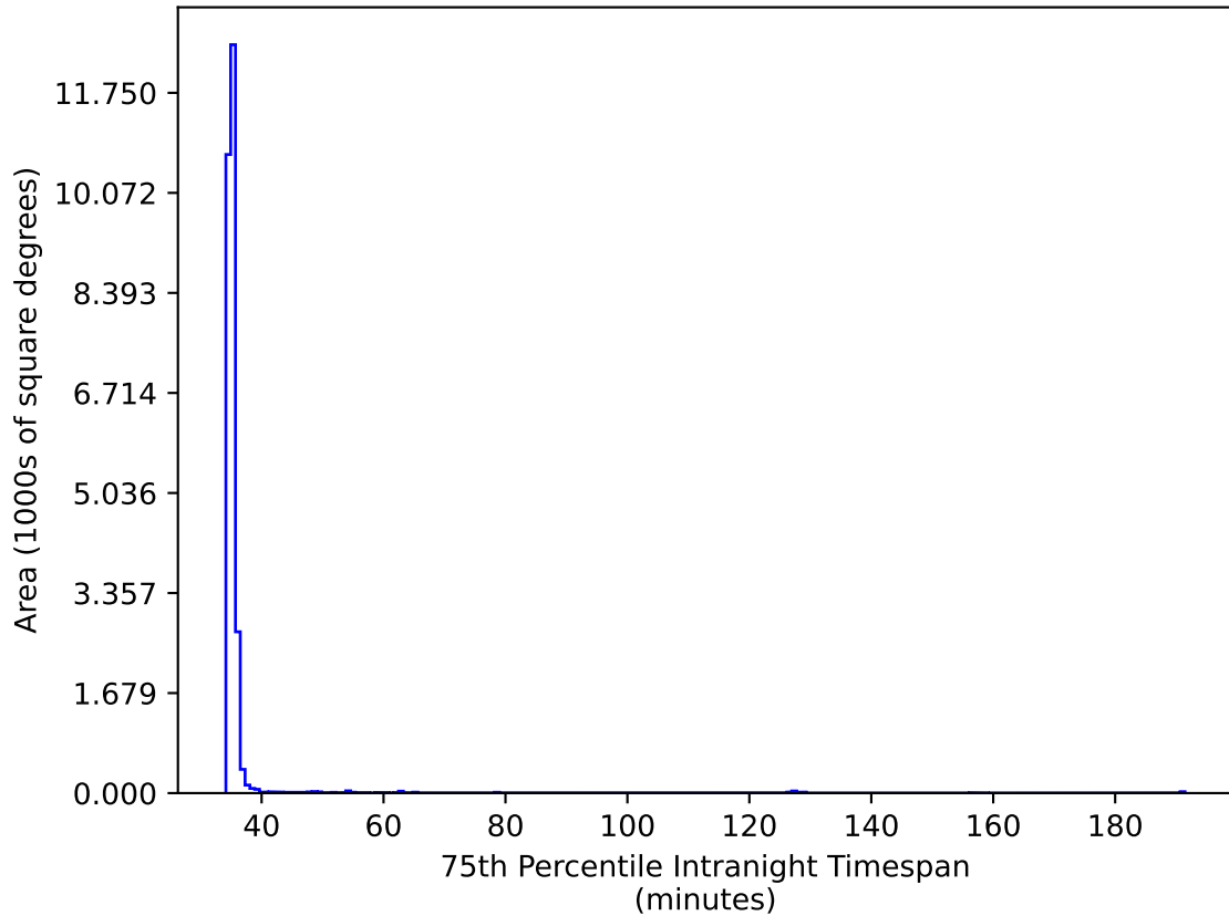
smc_lmc_v3.3_10yrs All sky iz bands: 75th Percentile Intranight Timespan
