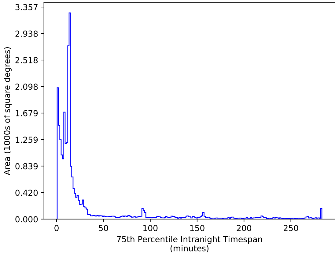
smc_lmc_v3.3_10yrs All sky i band: 75th Percentile Intranight Timespan
