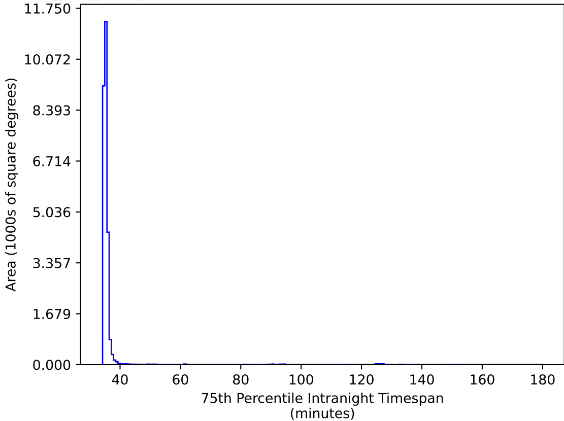
smc_lmc_v3.3_10yrs All sky gr bands: 75th Percentile Intranight Timespan
