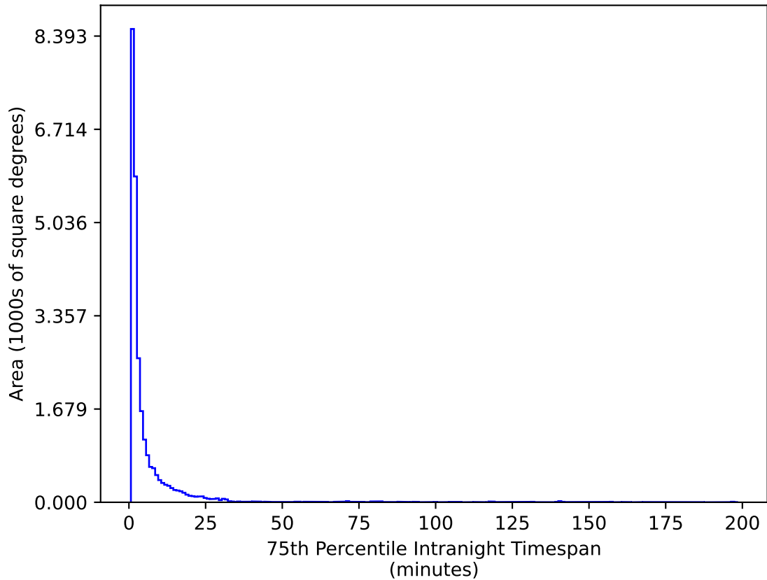
smc_lmc_v3.3_10yrs All sky g band: 75th Percentile Intranight Timespan
