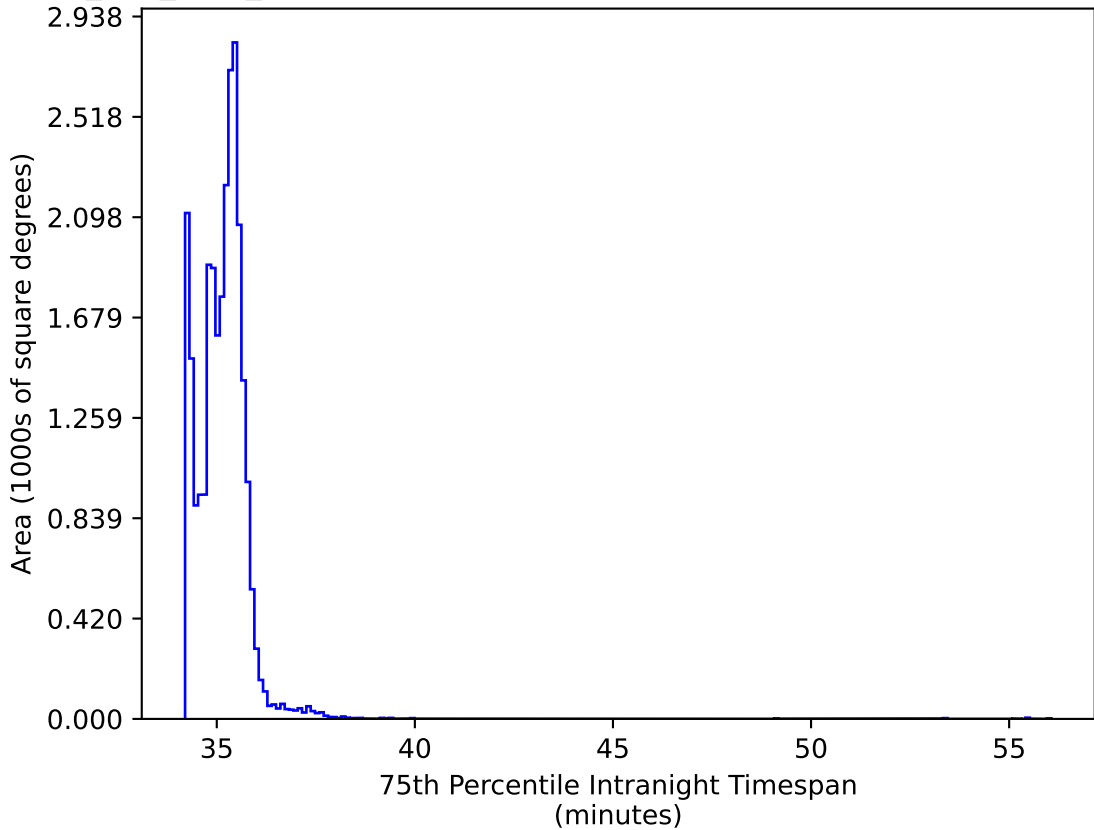
smc_Imc_v3.3_10yrs All sky all bands: 75th Percentile Intranight Timespan
